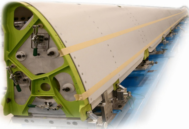
787 Fixed Leading Edge Wing Assembly
